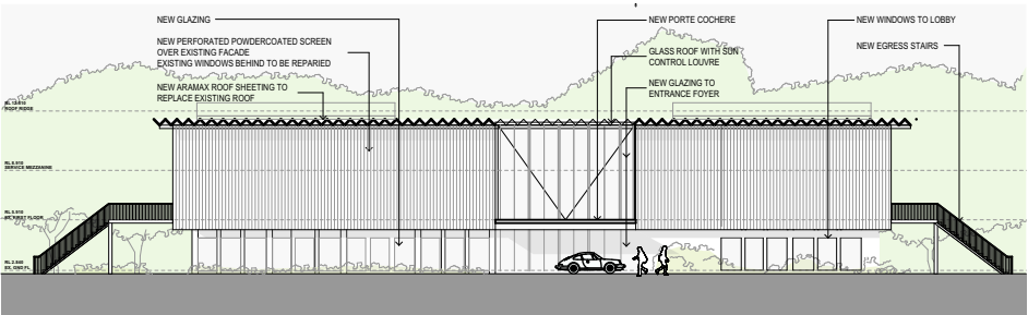
East Elevation - 1:500
