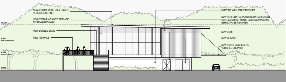
South Elevation - 1:500
